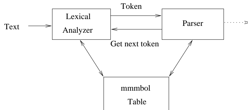
Figure 3.1 Interaction of lexical analyzer with parser
