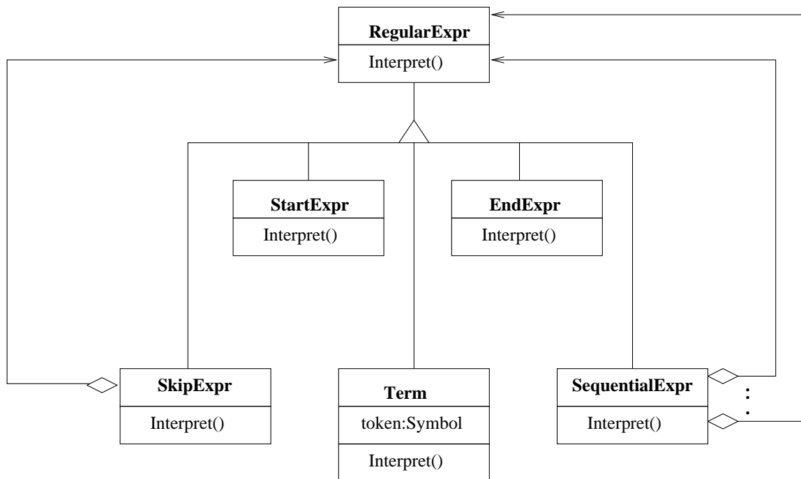
Figure 3.4 The Class Diagram for IEPlus Grammar
