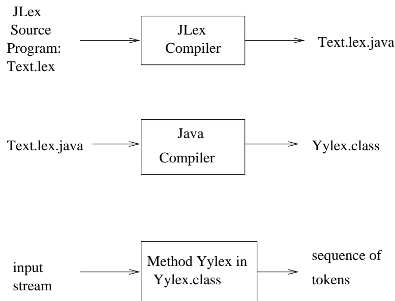
Figure 3.2 JLex Usage
