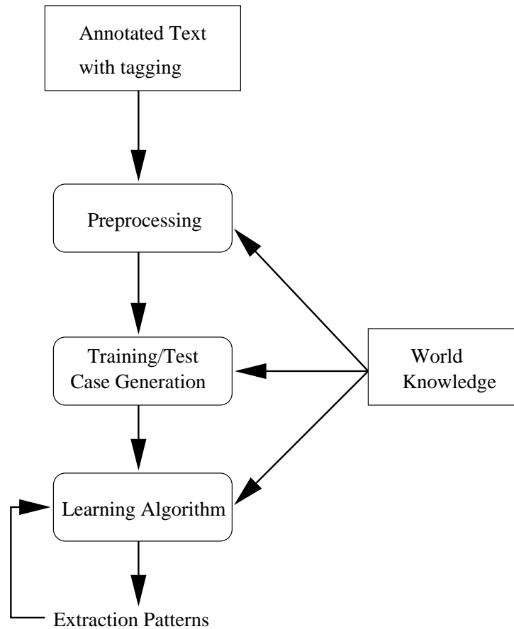
Figure 2.1 IE Extraction Pattern Learning Diagram
