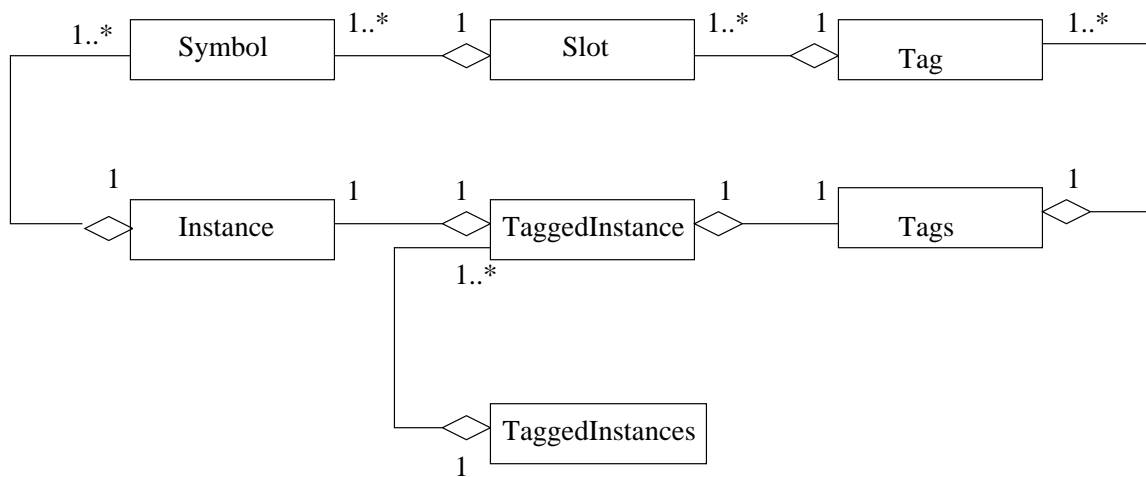
Figure 3.5 The Collection Class Diagram for IEPlus
