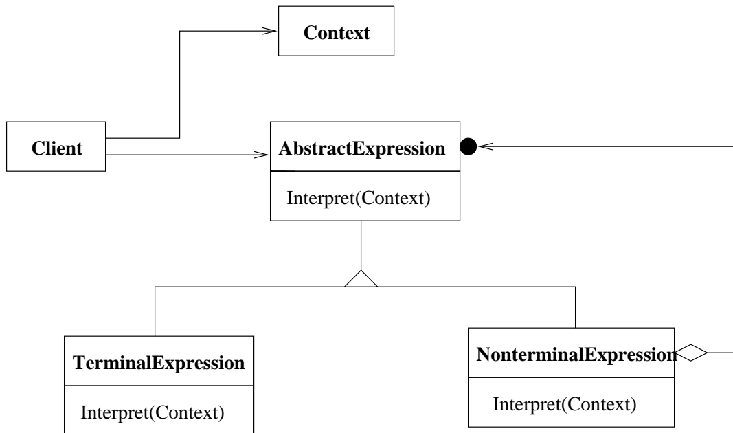
Figure 3.3 The Structure of Interpreter Design Pattern
