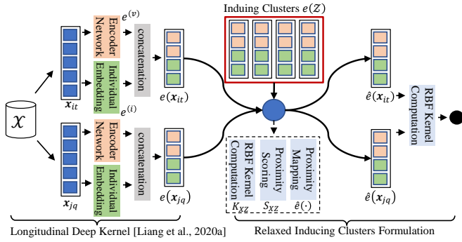
Figure 2: Graphical explanation of kernel computation in ICDCGP. The initial latent representation e(X) is computed the same way as in (Liang et al. 2021). The updated form of latent representation \hat{e}(X) is obtained by computing the proximity between the data points and inducing clusters, followed by the proximity mapping. The kernel value is computed based on the updated latent representation.
