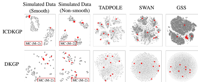
Figure 4: T-SNE visualization of the learned latent representation of ICDKGP and DKGP. The grey and the red dots represent the data points and the inducing cluster centers respectively.
