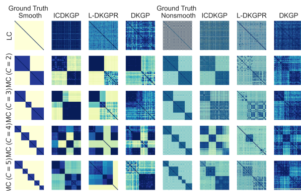
Figure 3: Recovering correlation structure: Comparison of ICDKGP with SOTA baselines on simulated data.
