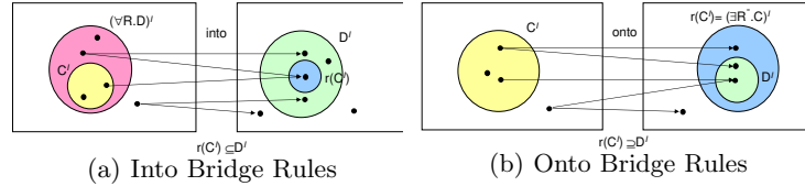
Fig. 1. Semantics of DDL Bridge Rules
