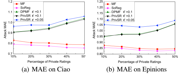
Figure 4: Privacy protection comparison.
