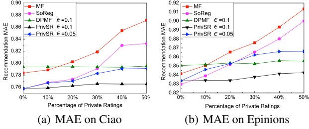
Figure 3: Recommendation effectiveness comparison.
