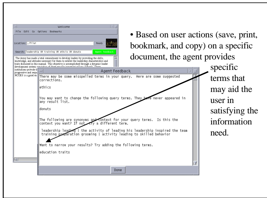
Figure 3: Interface for a specific implementation of AI 2 RS.
