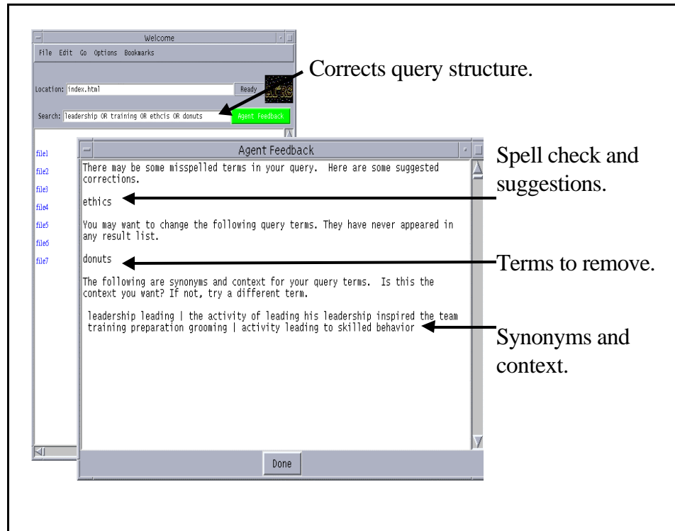
Figure 1: AI²RS agent interface and dialog box.
