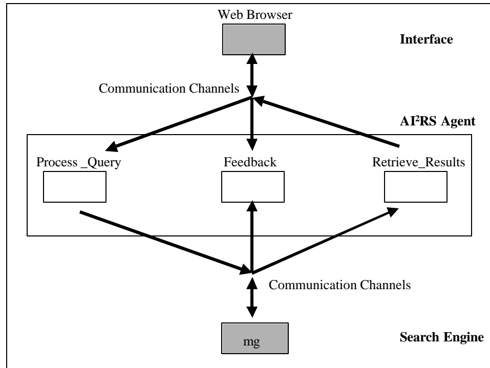
Figure 2: AI²RS modular structure.
