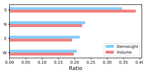
Figure 2: Learnt policy.
