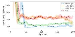
Figure 3: Ablation study.
